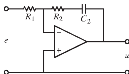
(a) PI controller
