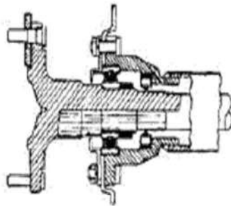
Fig..Semi-floatingball-race-bearing.
