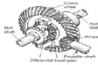
(d) Typical three-dimensional view
