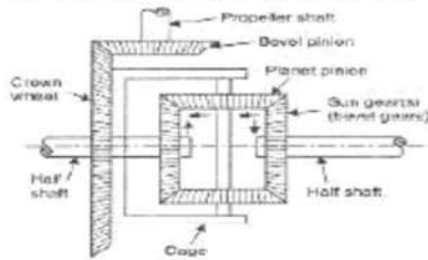
(c) Simple differential-simplified diagram
