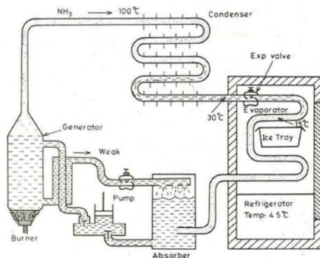
Vapor-Absorption Machine of Ferdinand Carre
