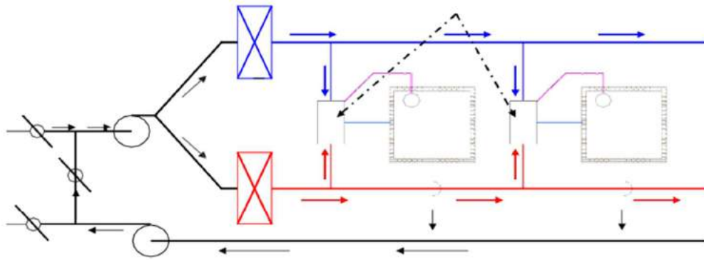
Dual duct, constant volume system
