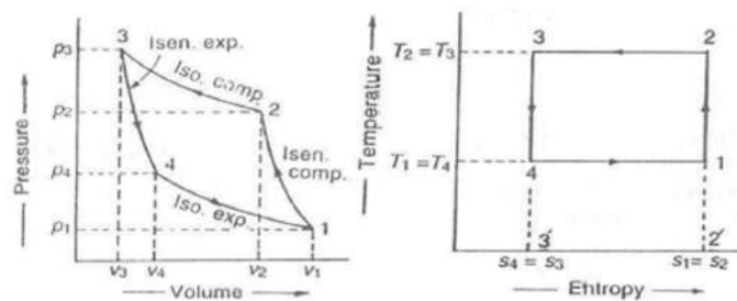
(a) p-v Diagram
