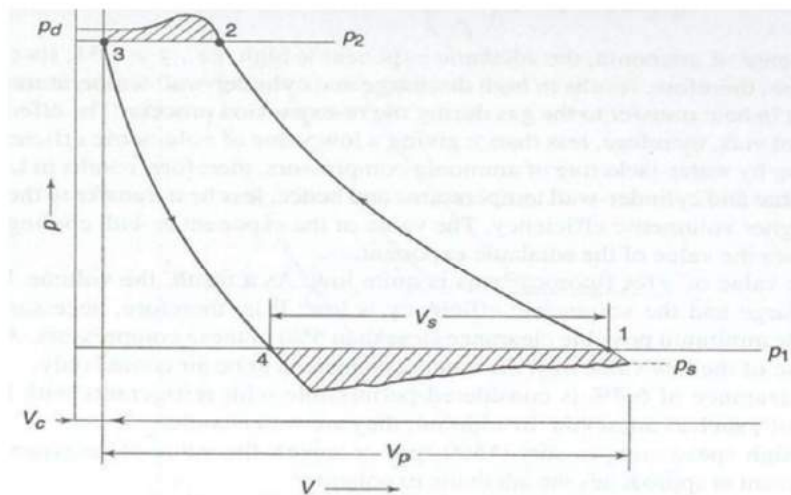
Effect of Valve Pressure Drops
