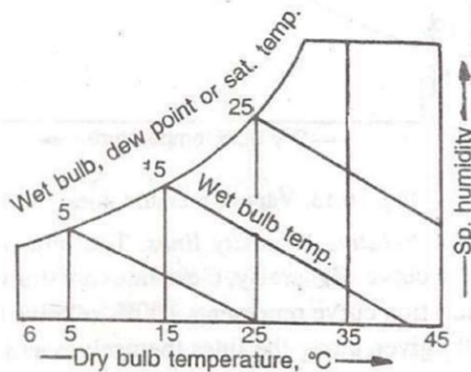
Wet Bulb Temperature Lines
