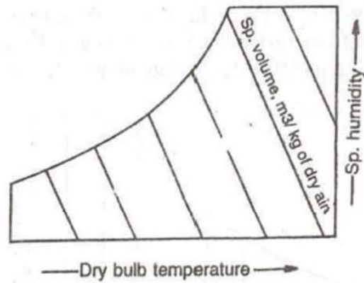
Specific Volume Lines
