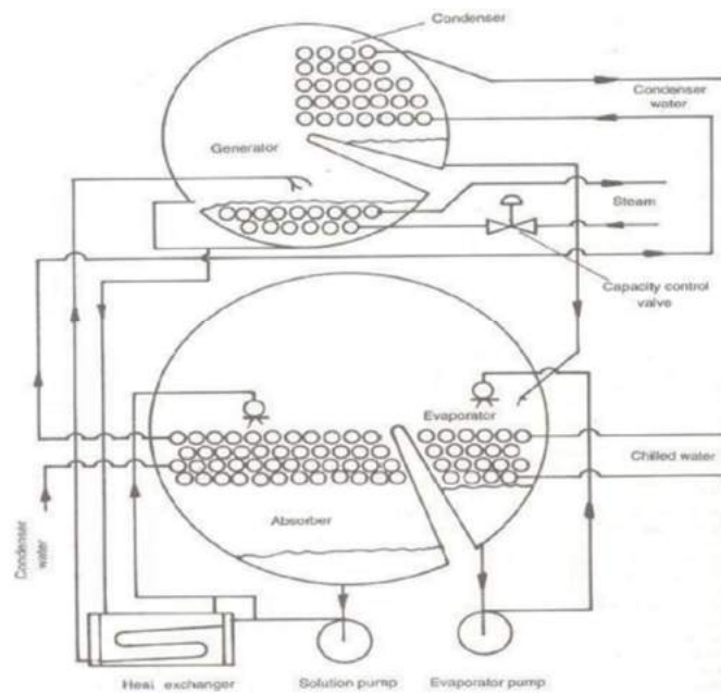
Schematic Diagram of Absorption System of Refrigeration
