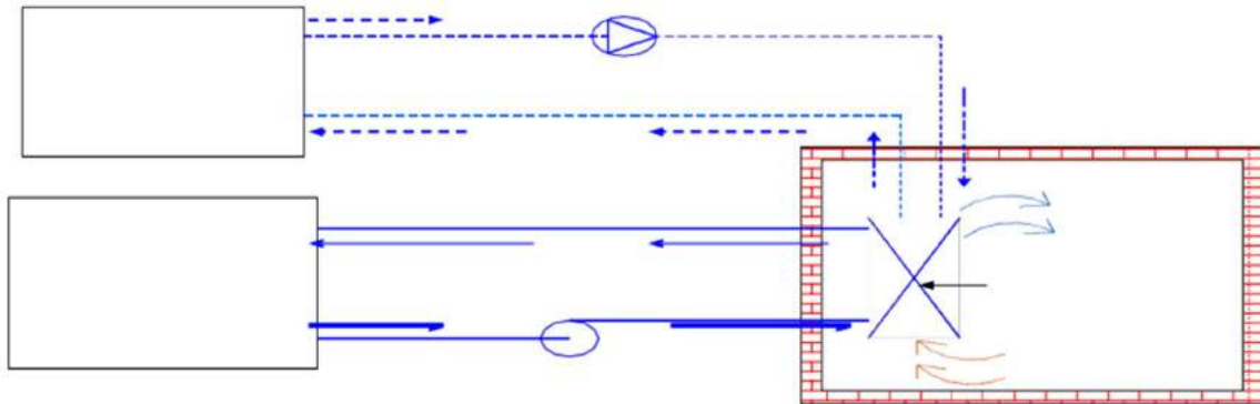
A basic air-water system
