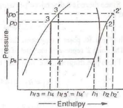
Effect of Discharge Pressure
