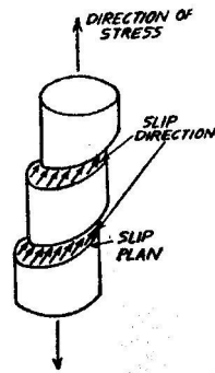
Fig. 3.2 Mechanism of slip Fig- 3.7
