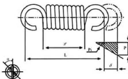
Tension
