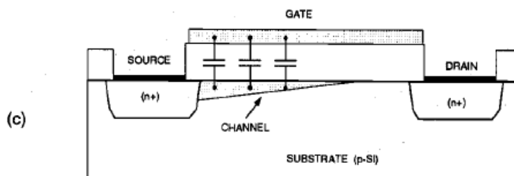
Figure..Schematic representation of MOSFET oxide capacitances during (a) cut-off, (b) linear, and (c) saturation modes.
