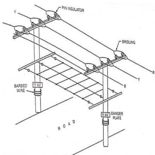
Cradle guard
