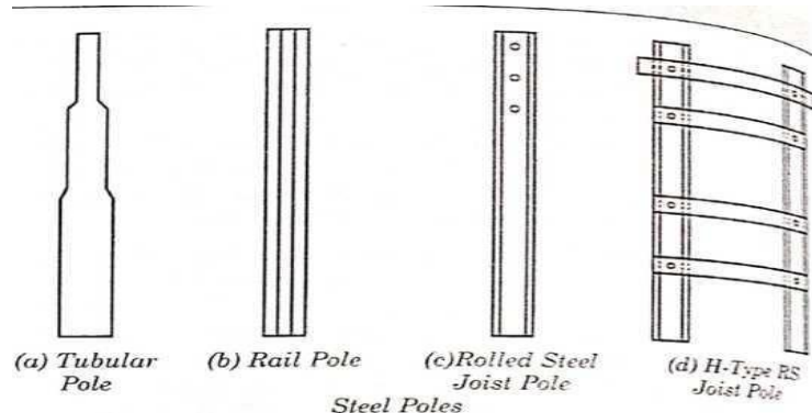
Steel Poles
