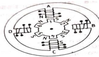
Fig. 9.51. Schematic Diagram of Stepper Motor.
