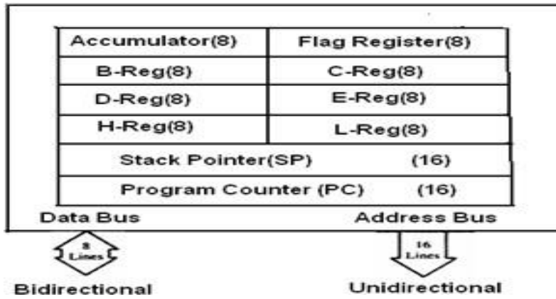
Fig. Register organization
