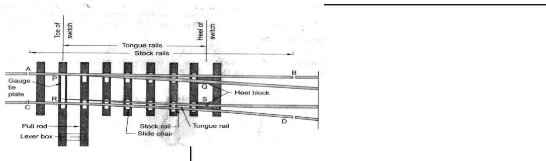
FIGURE: DETAILS OF SWITCH
