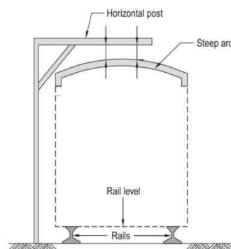
Fig. 2.2 Loading gauge
