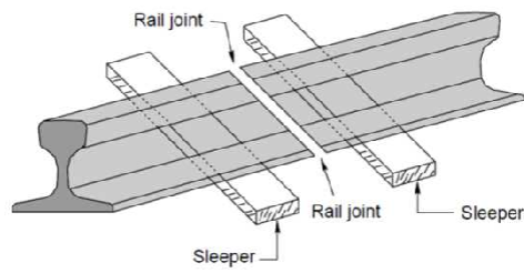
Suspended joint
