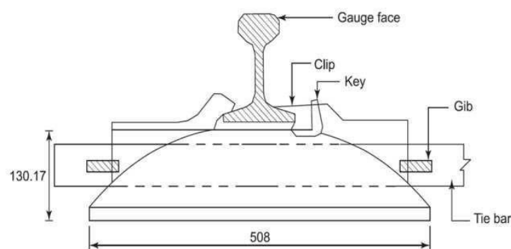
CI pot sleeper (dimensions in mm)
