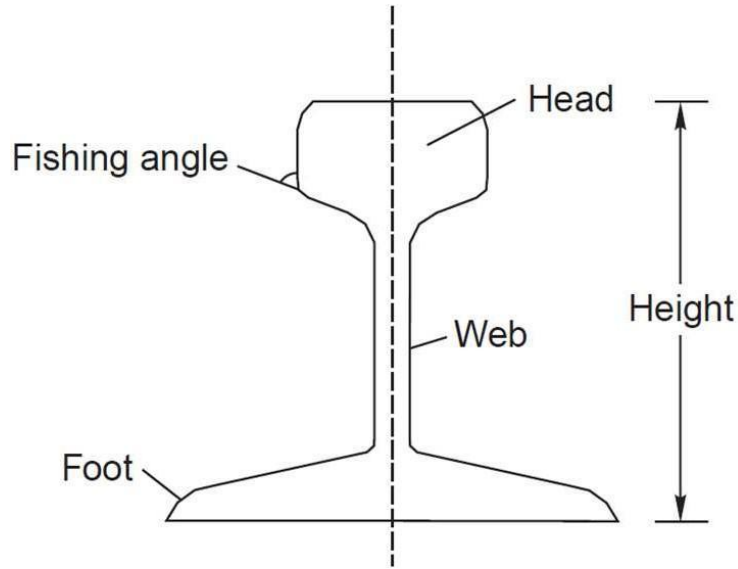
Flat-footed rail
