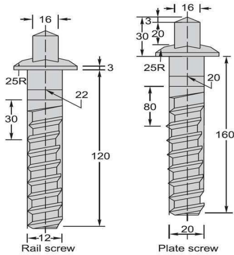
Screw spikes
