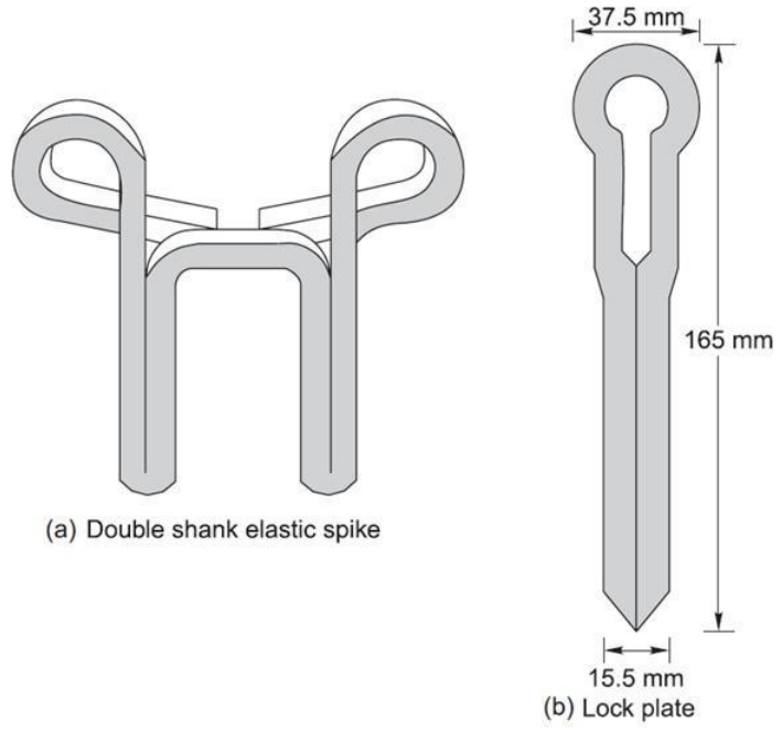
Lock spike
