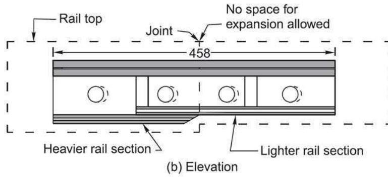
Combination fish plate (dimensions in mm)
