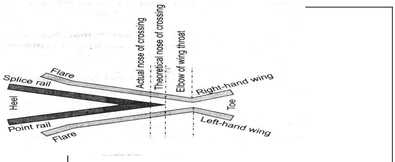
Figure: - Point Rail and Splice Rail
