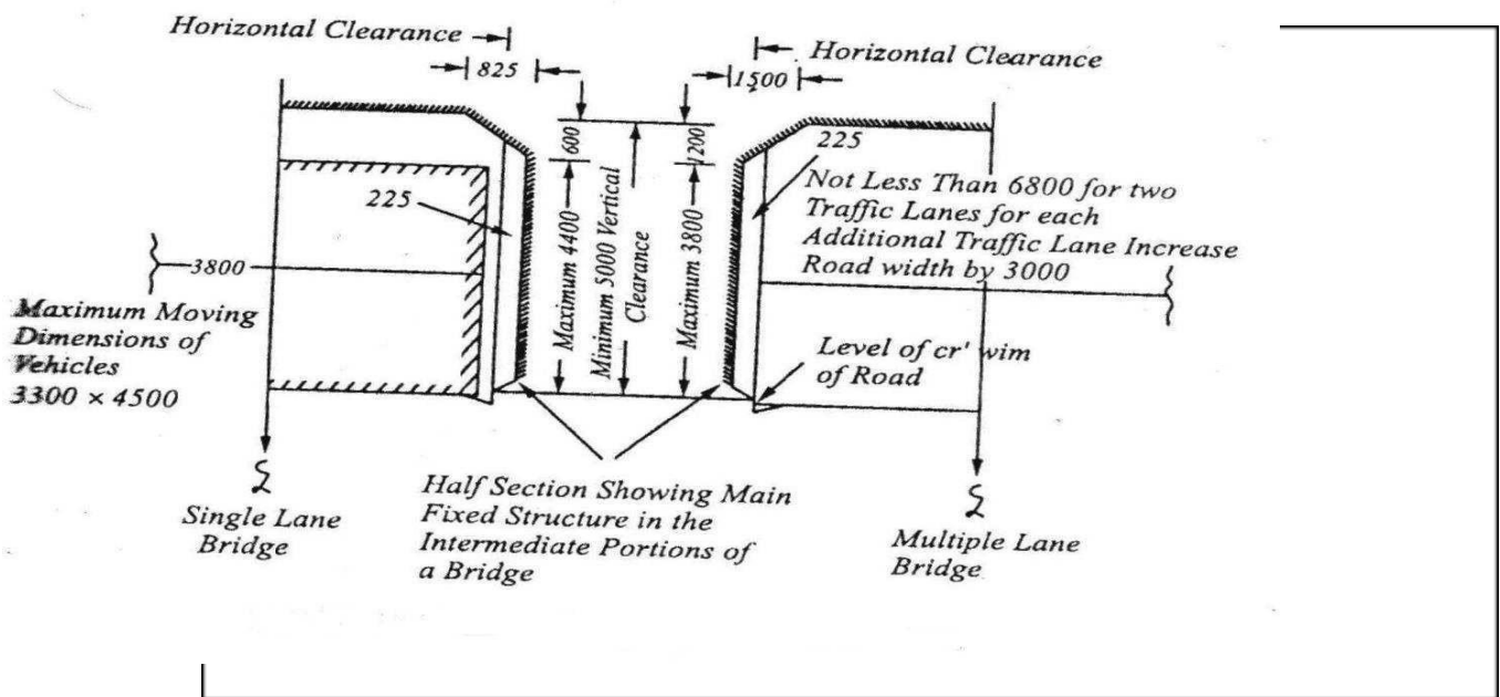
Clearance Diagram for Road Bridges
