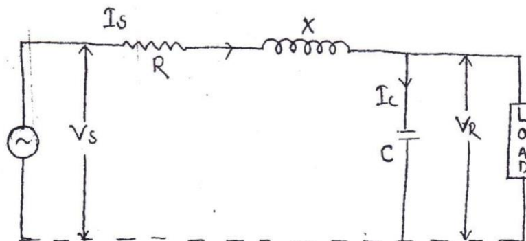
(Equivalent ckt for end condenser Method)
